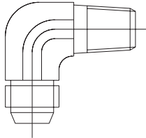
MALE ELBOW 1/8" NPT X 5/16" TUBING P/N: 69920503
