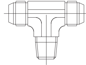
MALE BRANCH TEE 1/8" NPT X 5/16" TUBING P/N: 69920505
