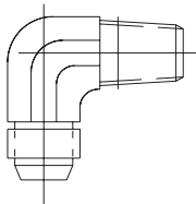
MALE ELBOW 1/8" NPT X 5/16" TUBING P/N 6992-0503
