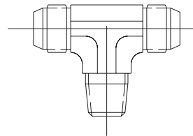
MALE BRANCH TEE 1/8" NPT X 5/16" TUBING P/N 6992-0505
