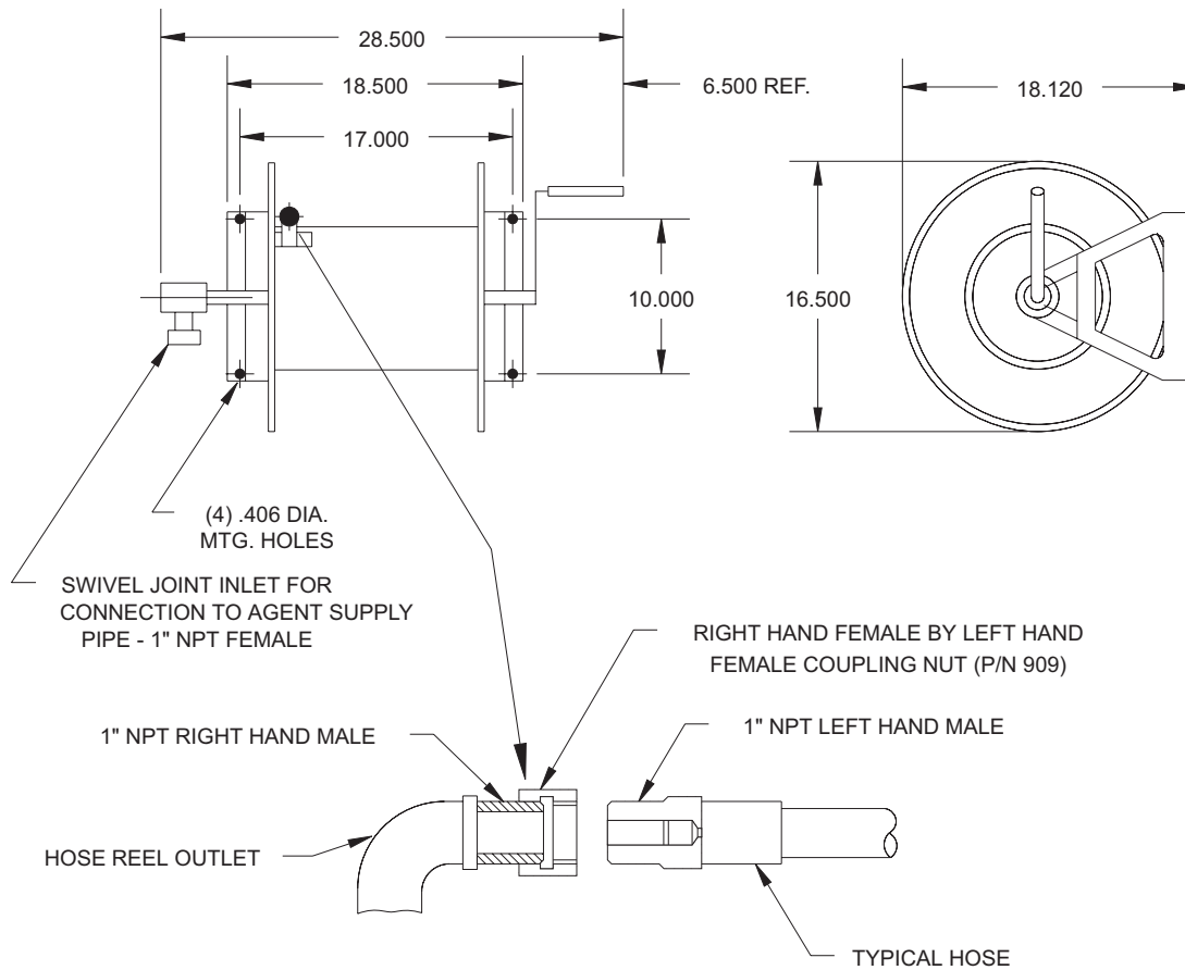
DETAIL - HOSE-TO-HOSE REEL CONNECTION
