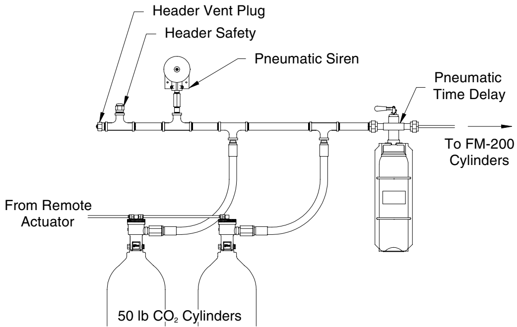
Typical Arrangement Marine FM-200 System
