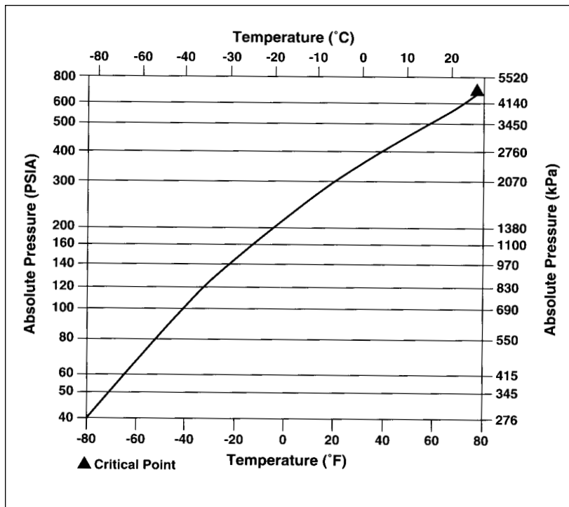
Figure 1. Saturated Vapor Pressure of FE-13
